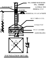
FOUNDATION DETAIL
