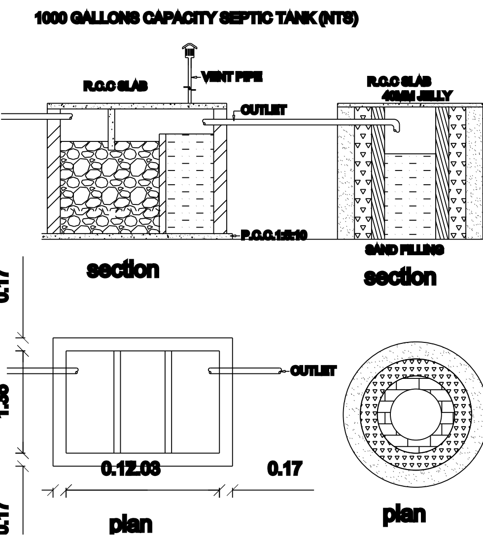
LEACH WELL DETAIL
