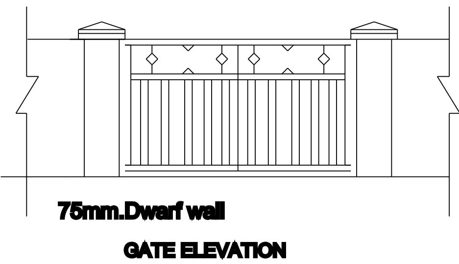
GATE ELEVATION
