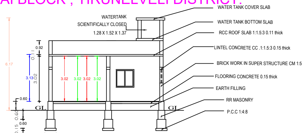
SECTION "A-B"
