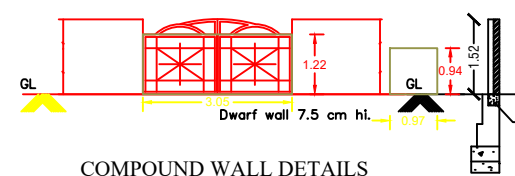
COMPOUND WALL DETAILS
