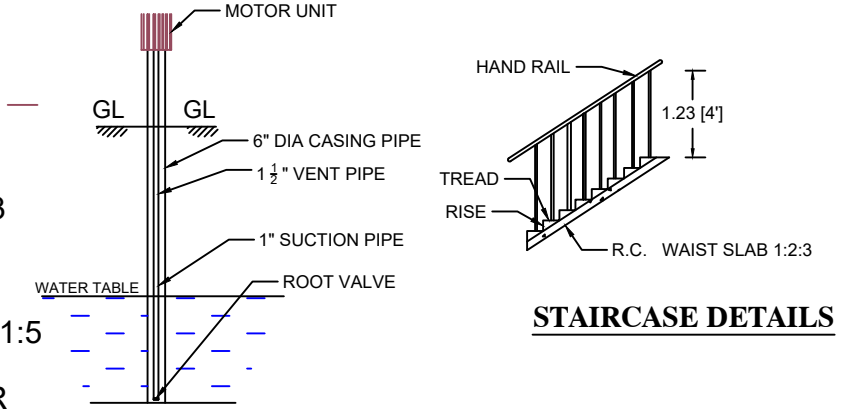
SEC.OF BOREWELL
