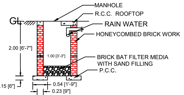
SECTION ON O - P
