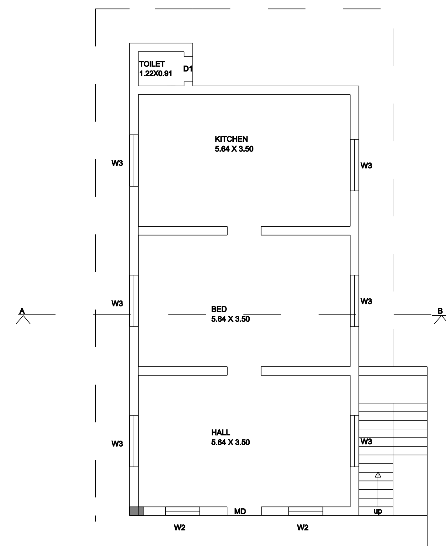
) FLOOR PLAN
