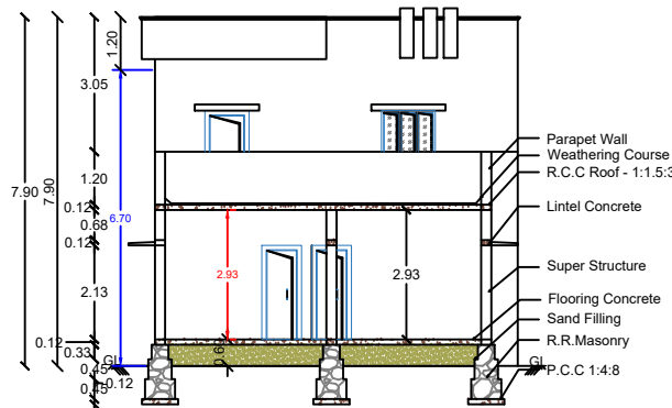
SECTION ON E-E
