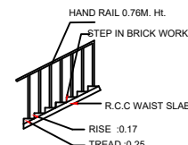
STAIR CASE DETAIL
