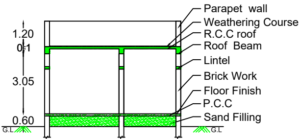
SECTION AB
