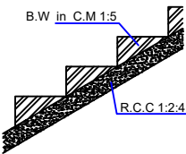
STAIRCASE
