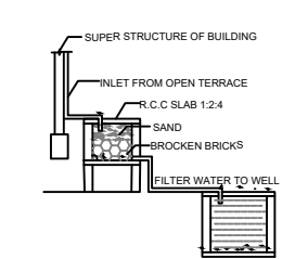
DETAILS OF FILTER BED & WELL NTS
