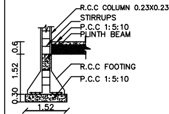
COLOUMN DETAILS
