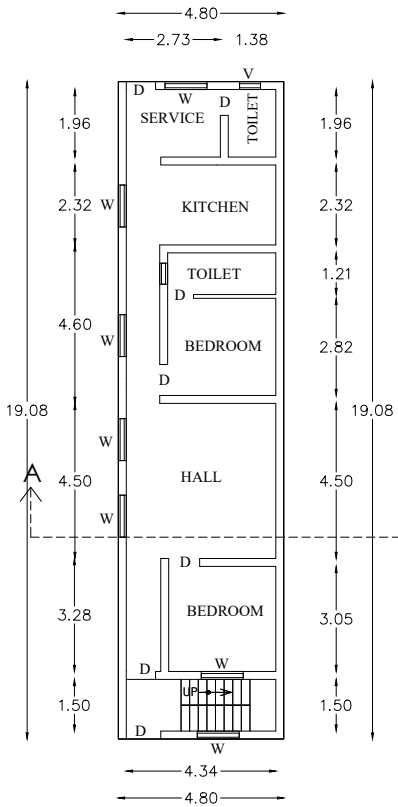
PRO GROUND FLOOR PLAN
