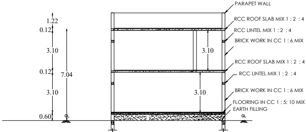
SECTION ON AB & ( HALF ELEVATION)
