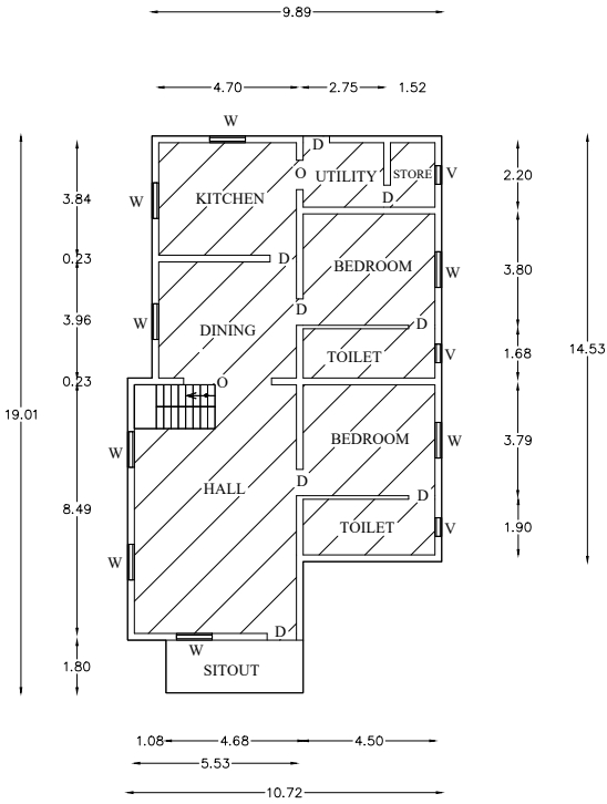
EXISTING GROUND FLOOR APPROVED PLAN
