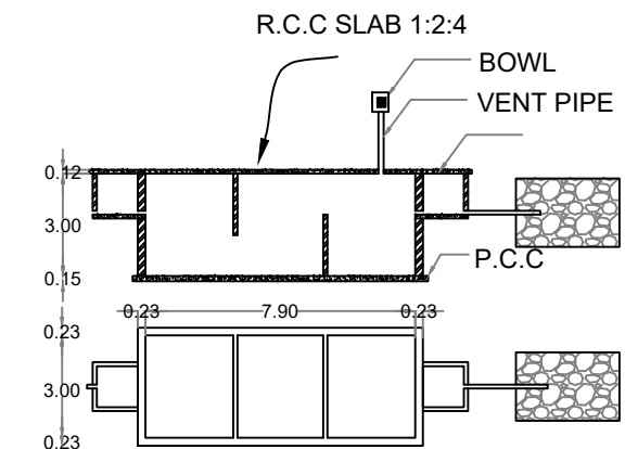
SEPTIC TANK AND TRENCH NTS
