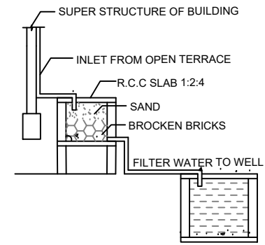
DETAILS OF FILTER BED & WELL NTS
