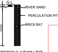
PERCULATION PIT
