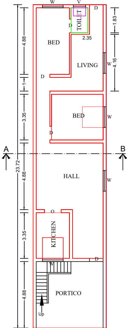
G.FLOOR PLAN
