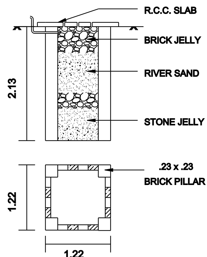
PLAN & SECTION OF RAIN WATER COLLECTION WELL
