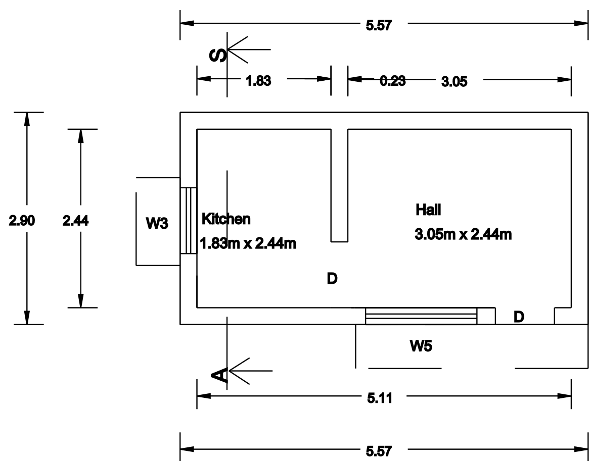
PLAN
