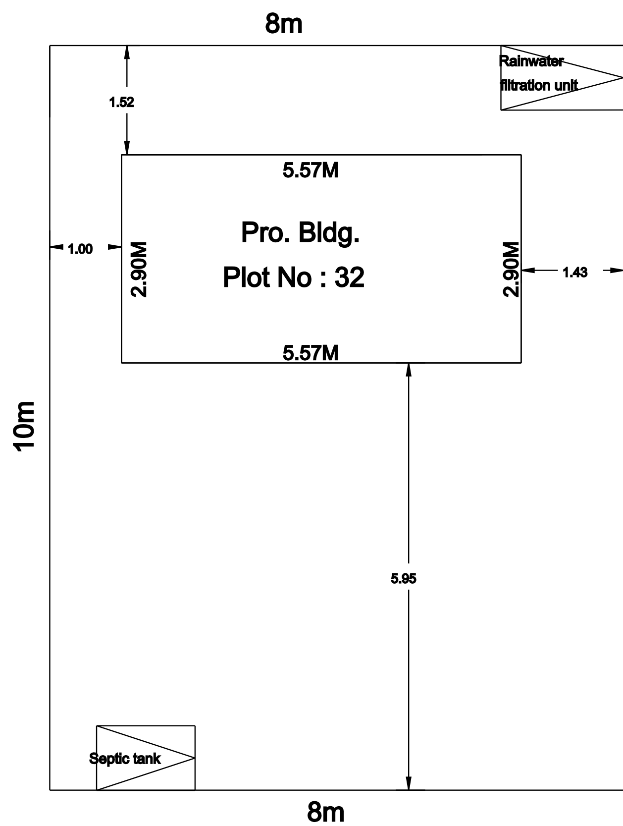
SITE PLAN
