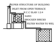
RAINWATER HARVESTING
