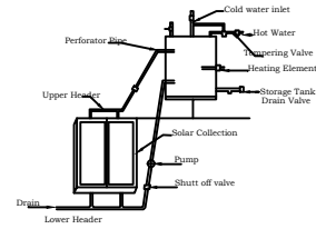
Details Of Solar Water Heater (NTS)
