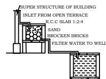
RAINWATER HARVESTING
