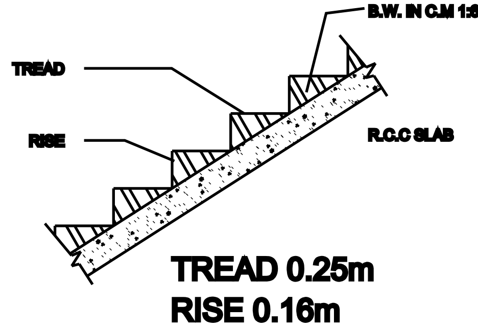
STAIR DETAILS
