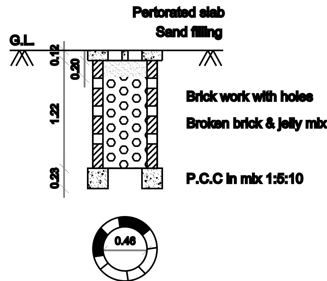
PERCOLATION PIT FOR 30 Sq. m.
