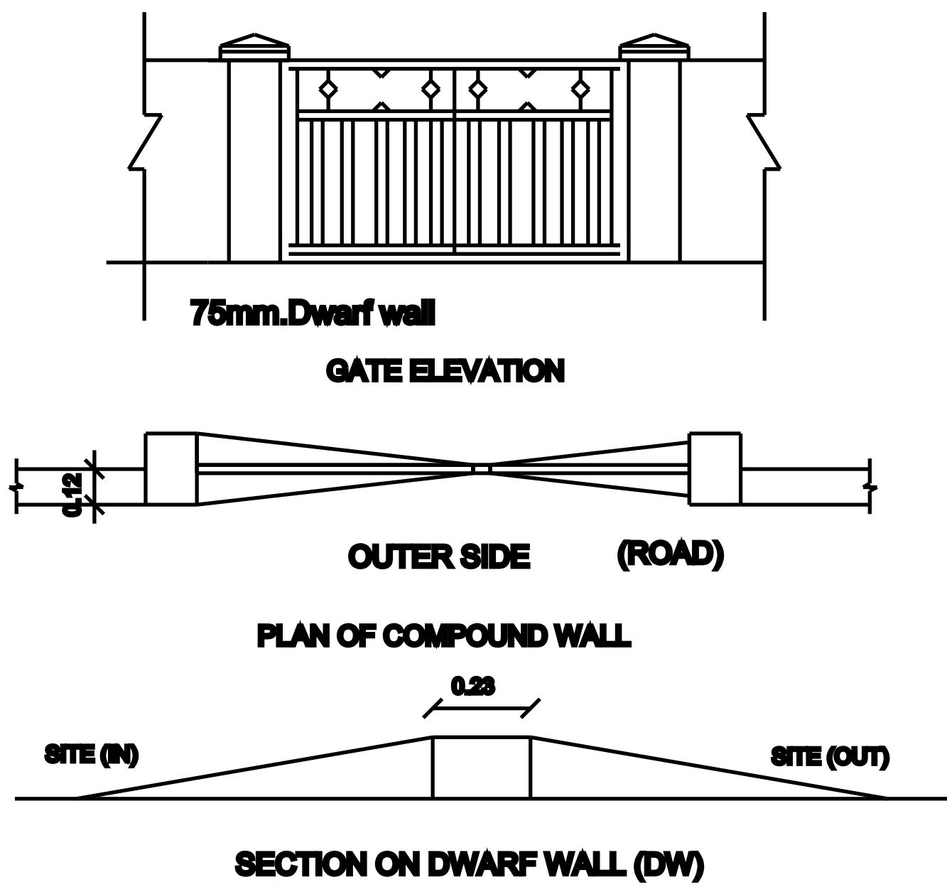
MAIN GATE DETAIL
