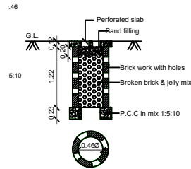
PERCOLATION PIT (Scale:- 1:50)
