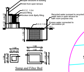
Sump and Filter Bed
