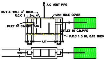
Septic Tank
