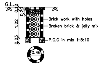
PERCOLATION PIT FOR 30 Sq. m. (Scale: - 1:50)
