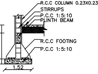
COLOUMN DETAILS
