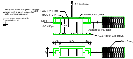
SEPTIC TANK AND TRENCH
