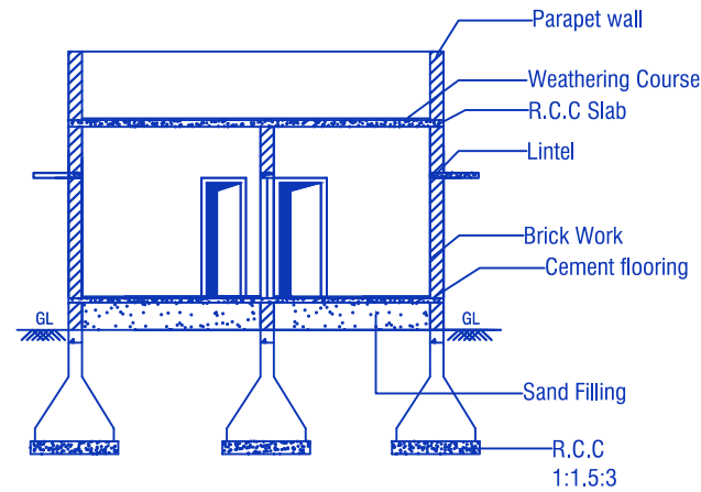
SECTION ON DWARF WALL (DW)
