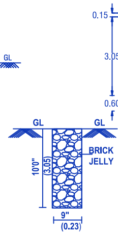
PERCULATION PIT
