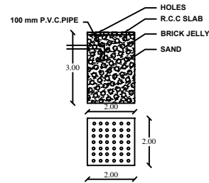
RAIN WATER COLLECTING TANK
