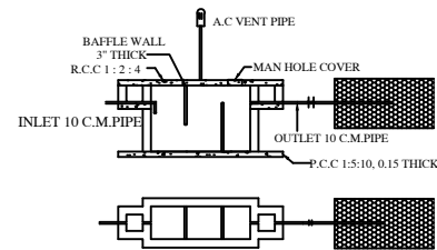
SEPTIC TANK & TRENCH
