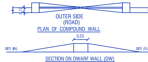
SECTION ON DWARF WALL (DW)
