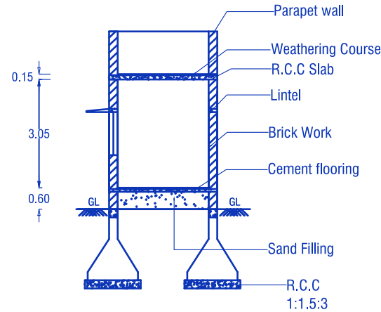
CROSS SECTION ON 'AB'
