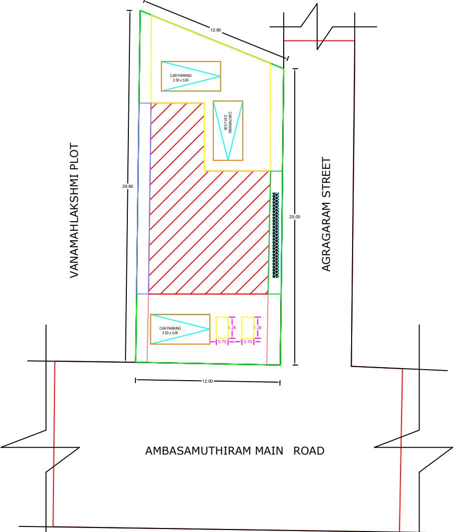
SITE PLAN
