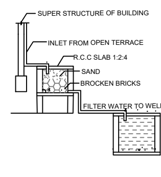
DETAILS OF FILTER BED & WELL
