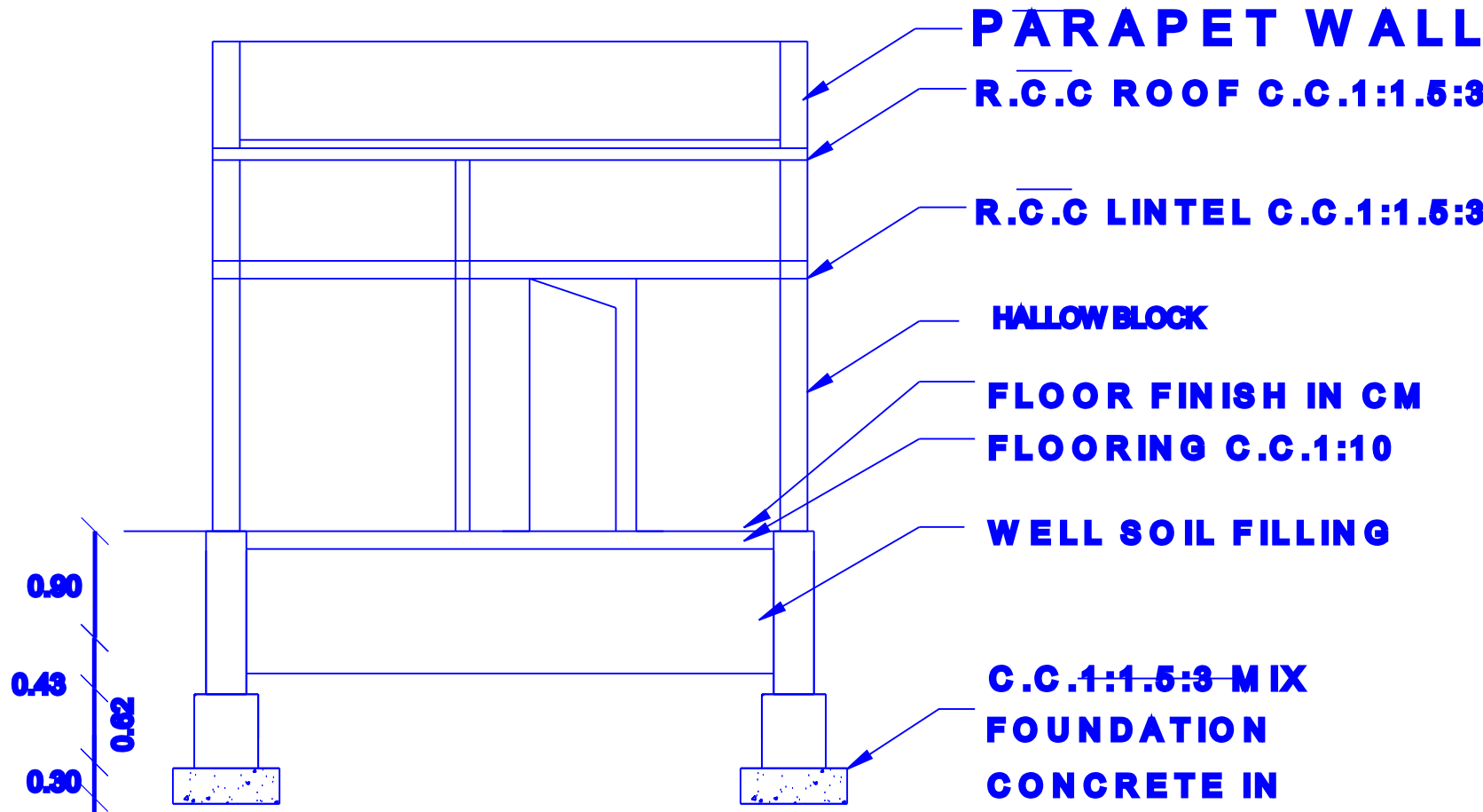
SECTION
