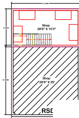
PLAN
