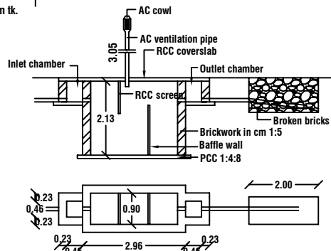
SEPTICTANK DETAILS
