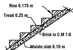
STAIR DETAILS
