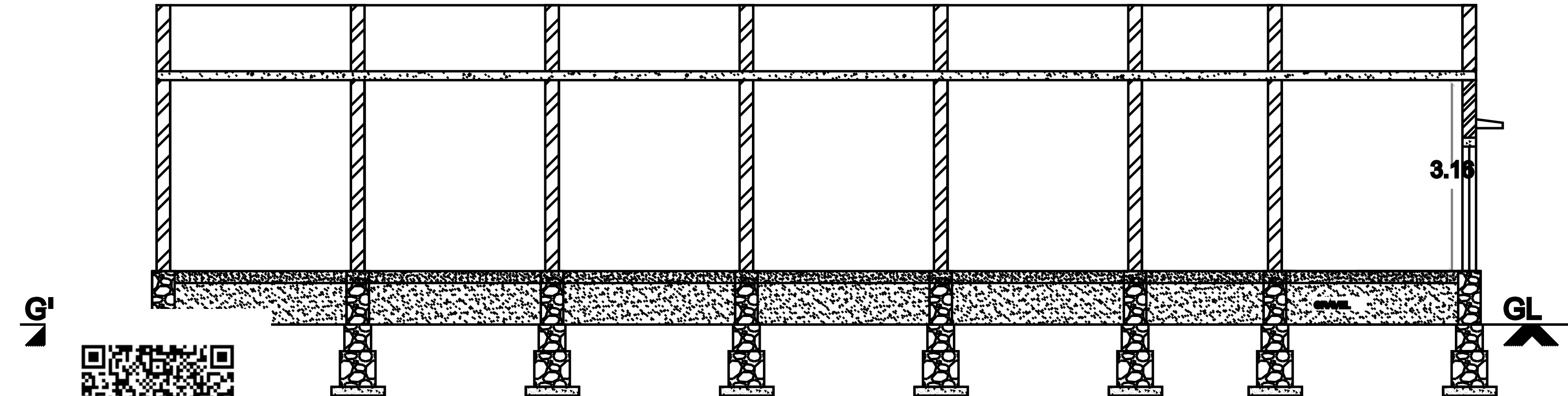
SECTION A
