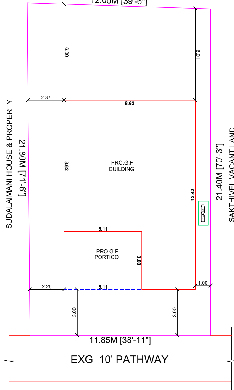
RAINWATER HARVESTING
