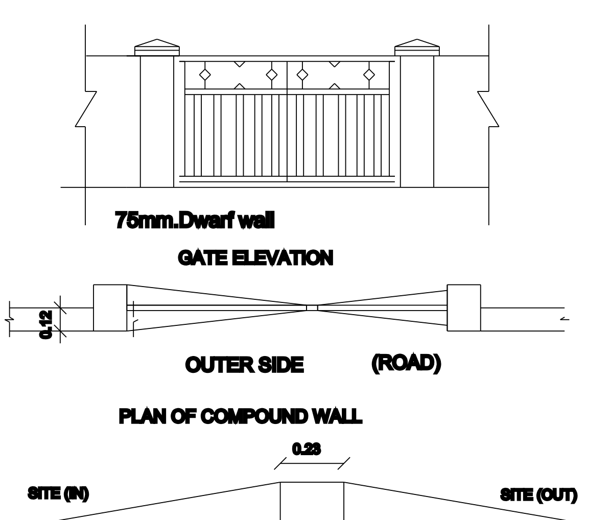
MAIN GATE DETAIL
