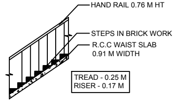
STEP DETAILS
