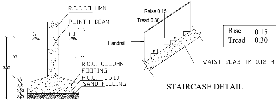
FOUNDATION DETAIL
