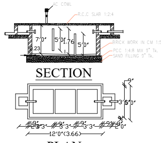
PLAN SEPTIC TANK DETAILS
