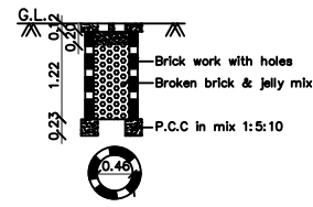
PERCOLATION PIT FOR 30 Sq. m. (Scale: - 1:50)
