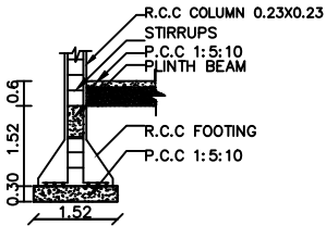
COLOUMN DETAILS
