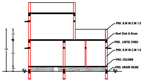
CROSS SECTION ON XX
