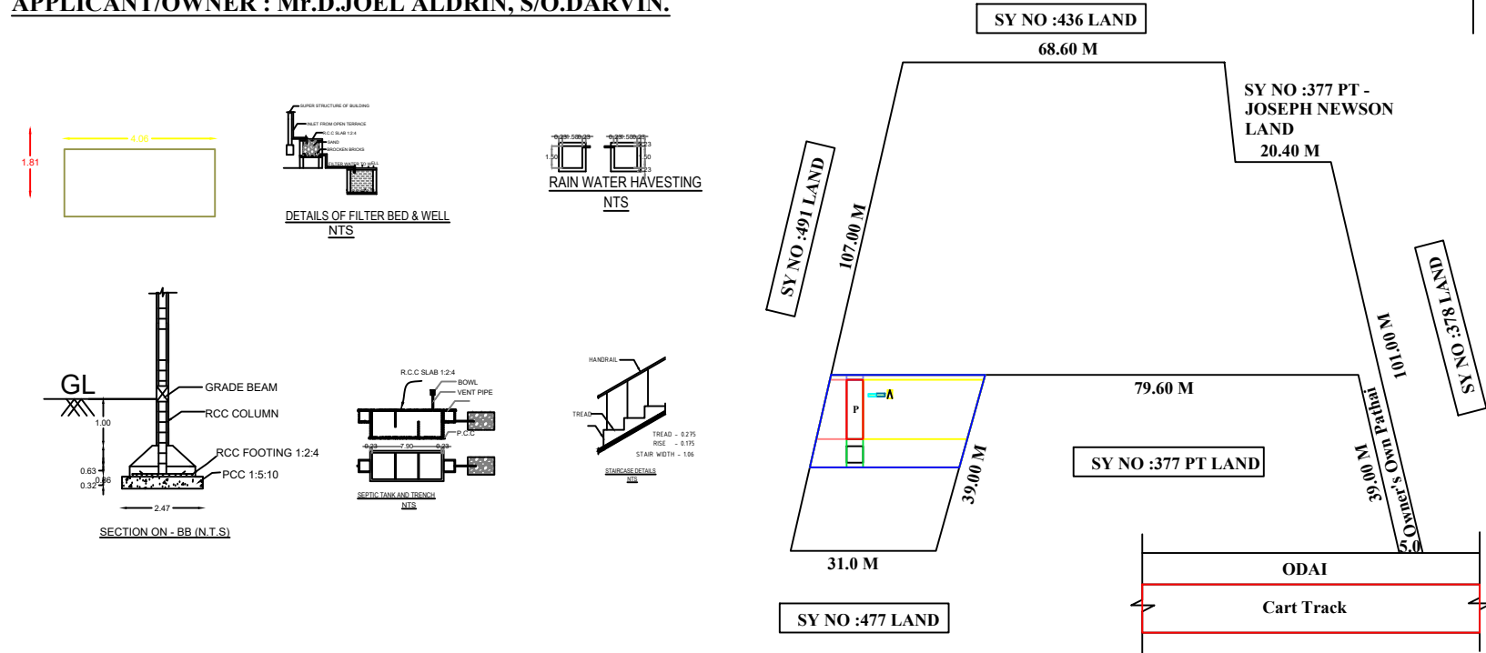
SITE PLAN
