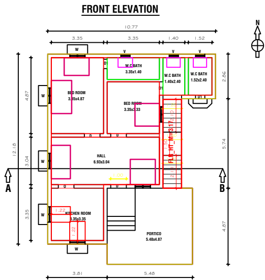
PRO GROUND FLOOR
