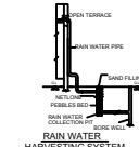
RAIN WATER COLLECTING SYSTEM
