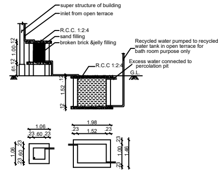
Sump and Filter Bed
