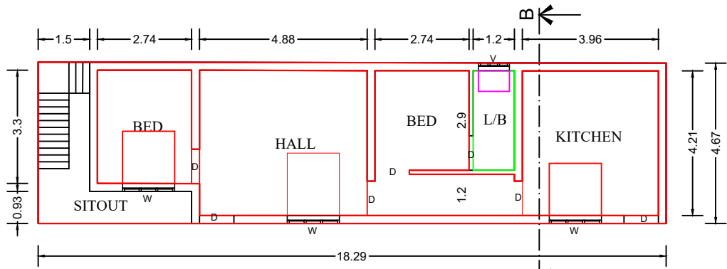
G.FLOOR PLAN
