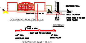
COMPOUND WALL PLAN
