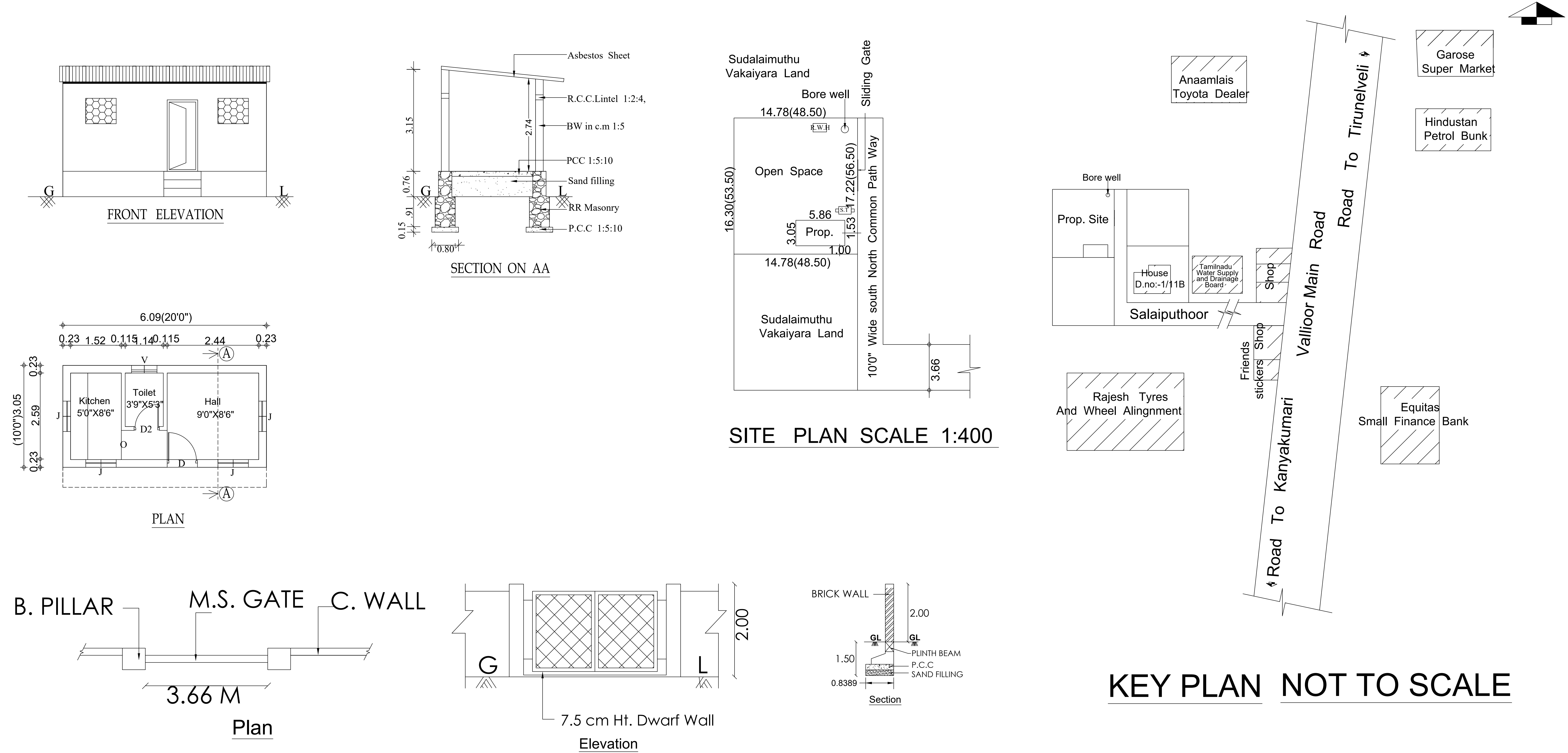
Compound Wall & Gate Details
