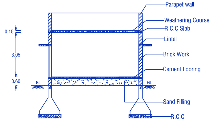
CROSS SECTION ON 'AB'
