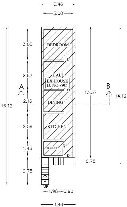
EX GROUND FLOOR PLAN
