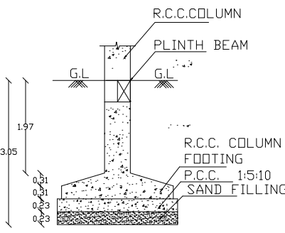
FOUNDATION DETAIL
