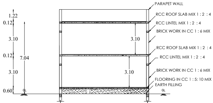
SECTION ON AB & ( HALF ELEVATION)
