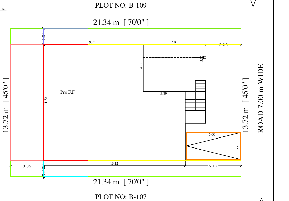
SITE PLAN
