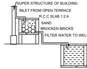
RAINWATER HARVESTING
