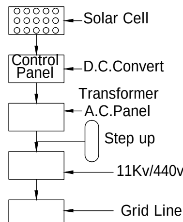
SOLAR SYSTEM
