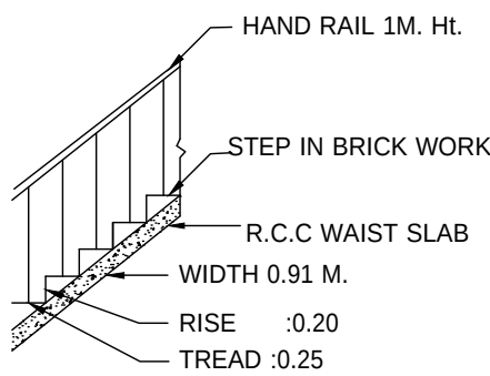
STAIR DETAIL
