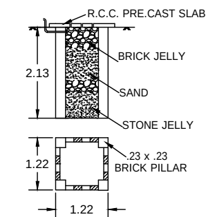
PLAN & SECTION OF RAIN WATER COLLECTION WELL
