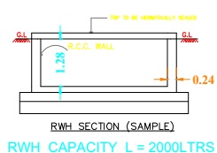
RWHS SECTION (SAMPLE) RWHS_CAPACITY_L = 2000LTRS
