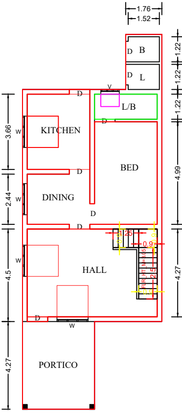
KEY PLAN
