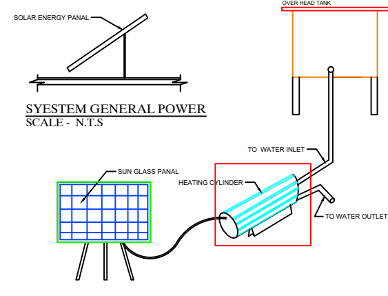
SOLAR WATER HEATING SYSTEM SCALE - N.T.S
