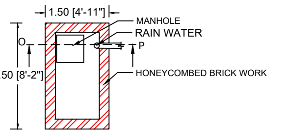
PLAN RAIN WATER HARVESTING
