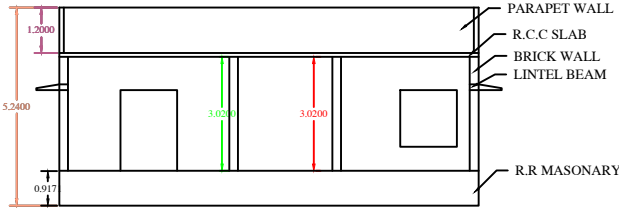
SECTION AT X-X'
