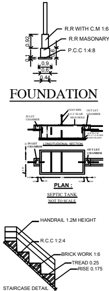
STAIRCASE DETAIL
