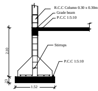
Column Detail
