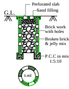
PERCOLATION PIT (NOT FOR SCALE)
